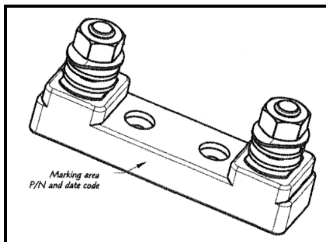
Fig. 4 - Fuse Holder ECS0858-XXX marking location
