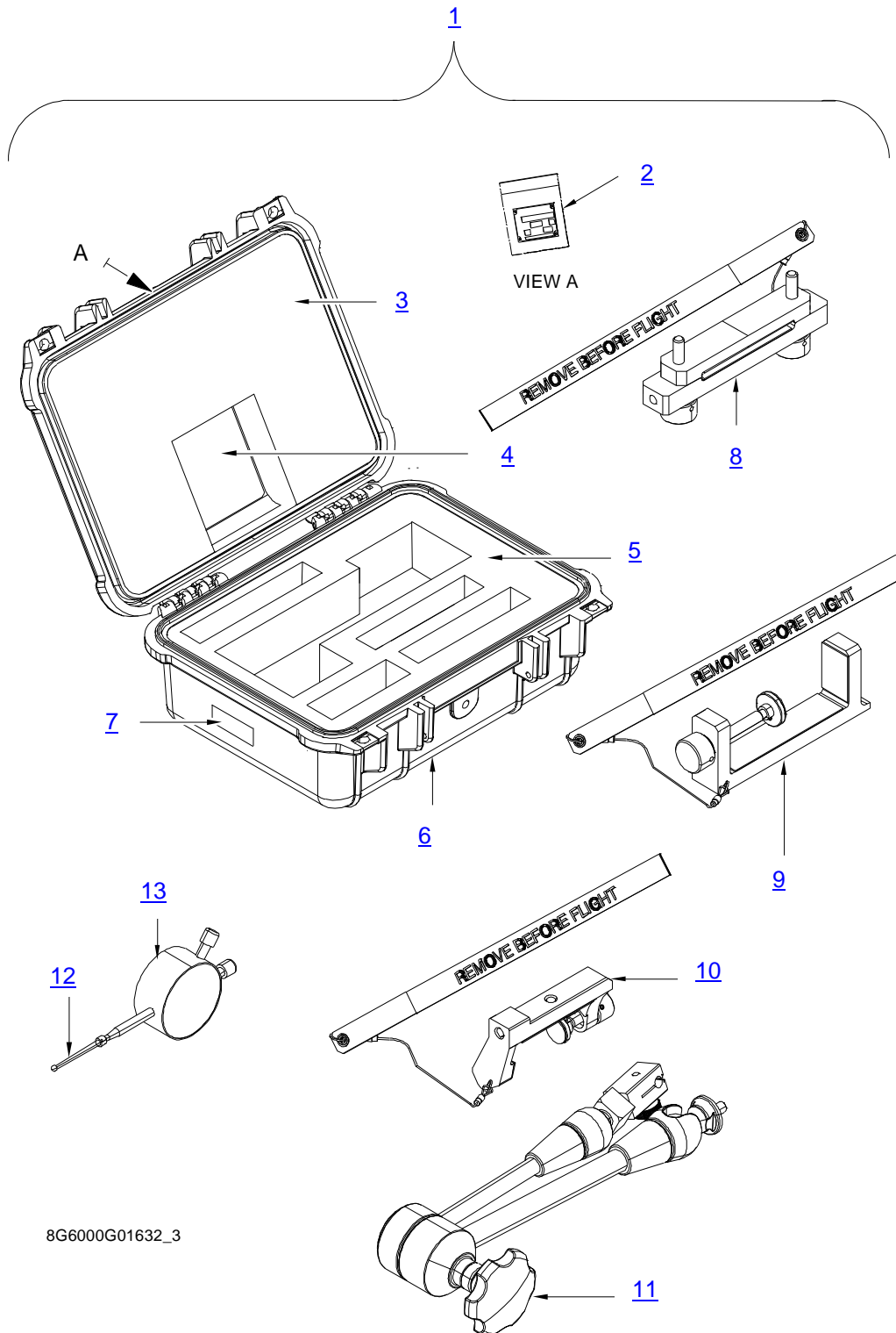
Figure 5 – Spare Parts
