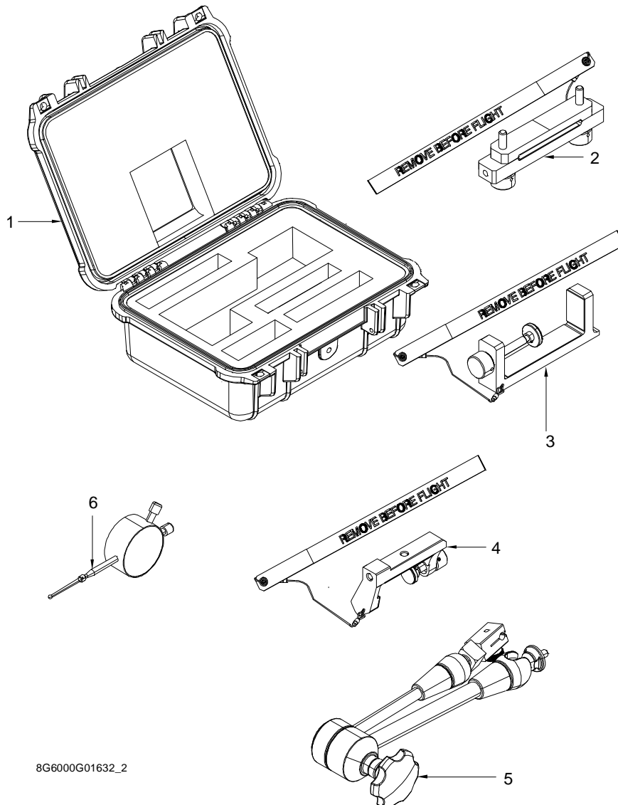
Figure 3 – Main Parts
