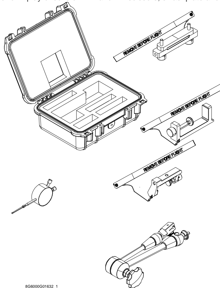
Figure 1 – Tool kit, rotors play check.
