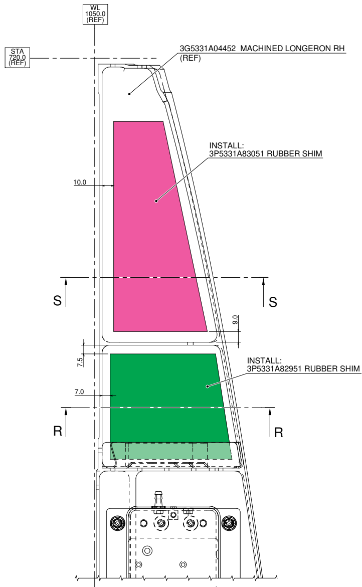
VIEW Q 3G3040L00151 RESERVOIR IS OMITTED FOR CLARITY STRUCTURES AND SYSTEMS ARE PARTIALLY OMITTED FOR BETTER CLARITY PURPOSE
