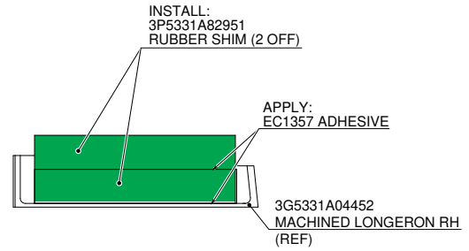
SECTION R-R STRUCTURES AND SYSTEMS ARE PARTIALLY OMITTED FOR BETTER CLARITY PURPOSE
