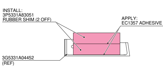
SECTION S-S STRUCTURES AND SYSTEMS ARE PARTIALLY OMITTED FOR BETTER CLARITY PURPOSE
