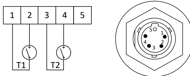
Connector Pinout Figure 1002
