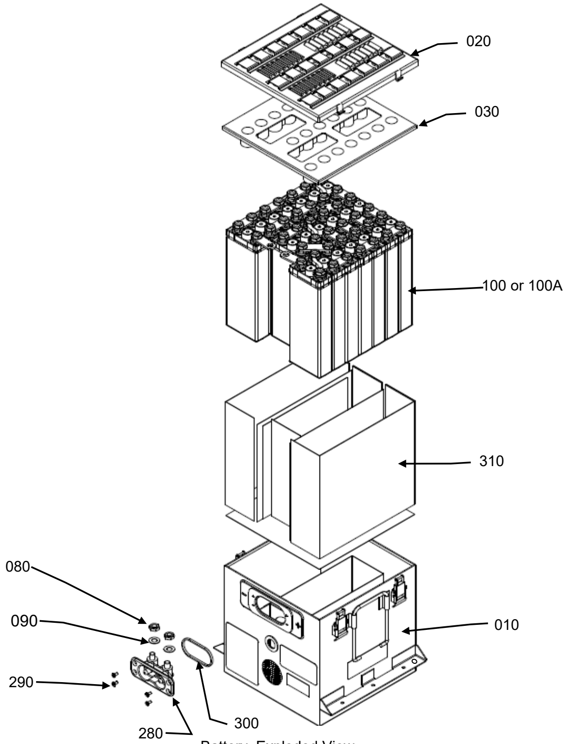
Battery, Exploded View IPL Figure 1 (#1 of 4)
