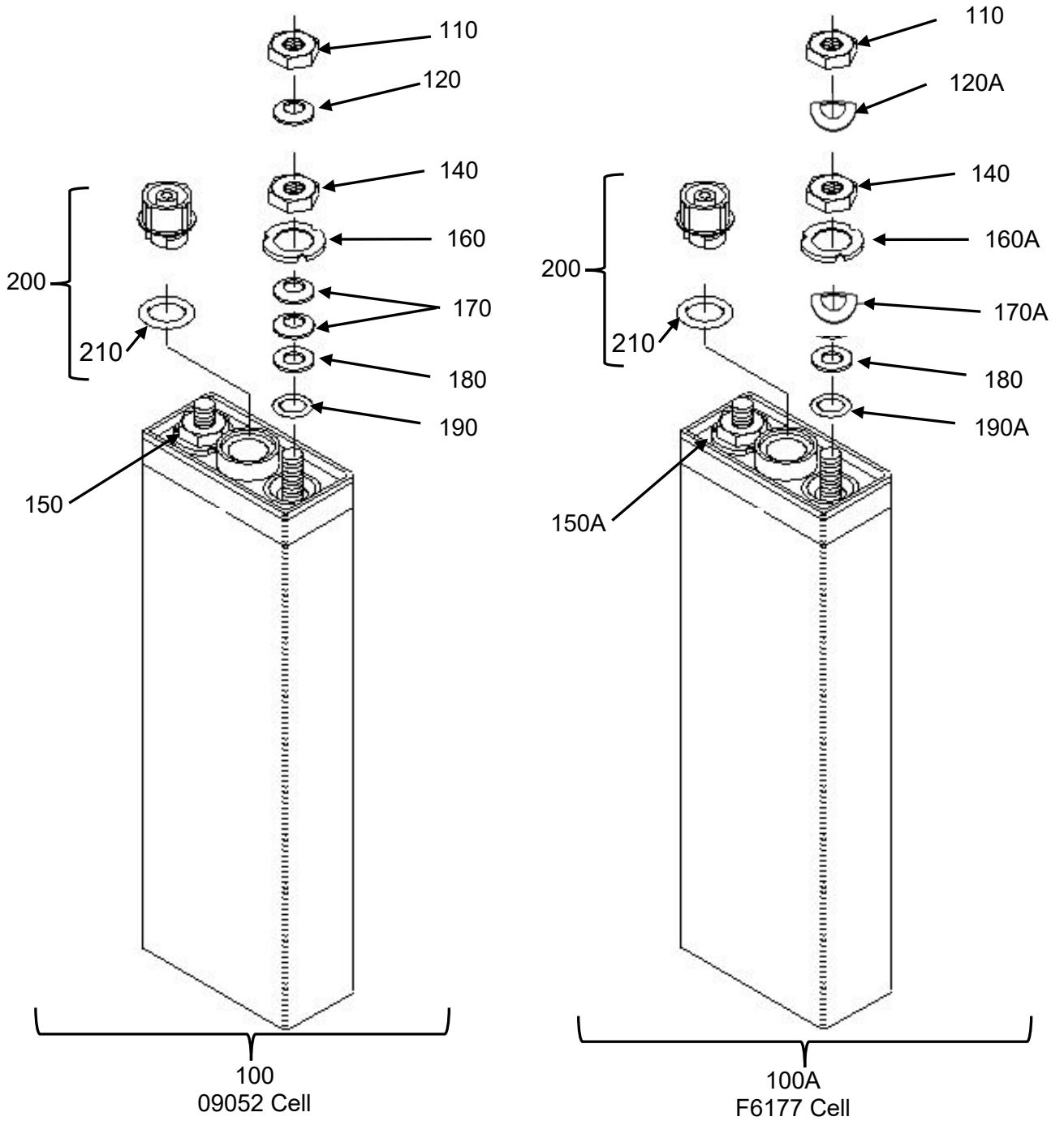
Battery, Exploded View IPL Figure 1 (#2 of 4)
