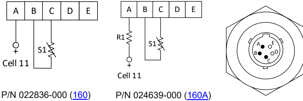
Connector Pinout Figure 1005
