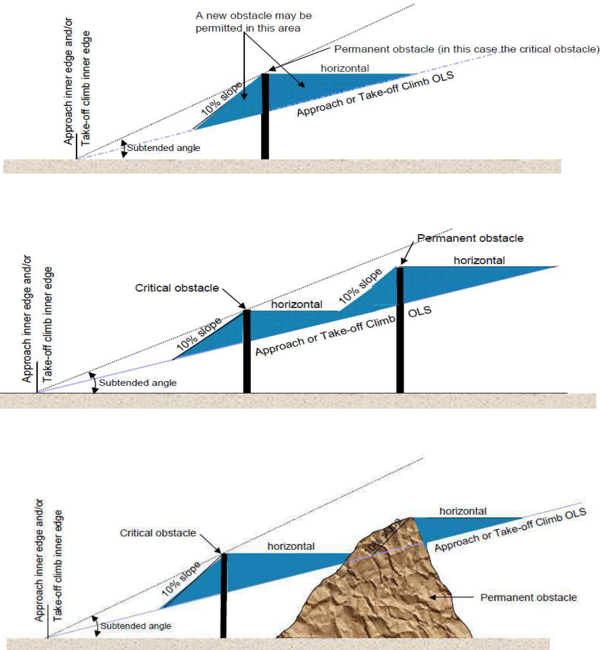
Figure 6-1: Shielding of obstacles penetrating the approach and take-off climb surfaces
