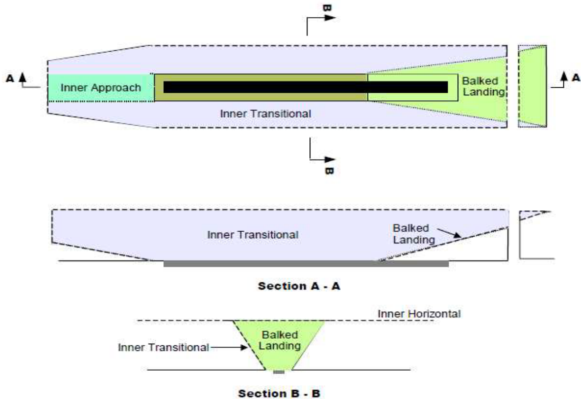
Figure 3-2: Inner approach, inner transitional and balked landing obstacle limitation surfaces
