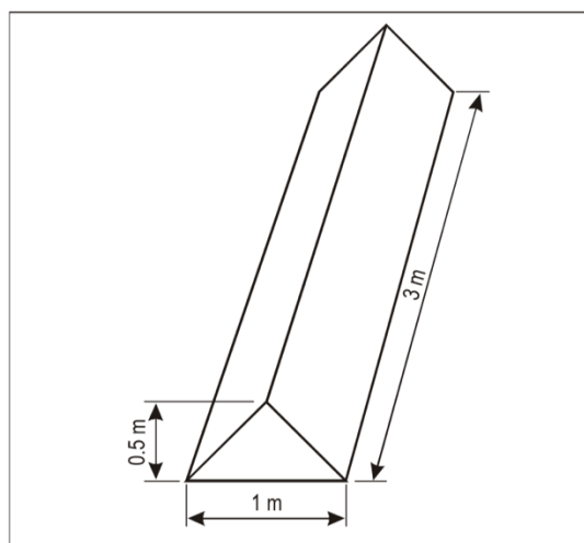
Figure 5-34. Boundary marker
