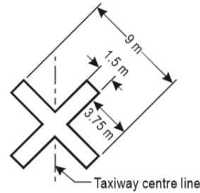
Illustration b) Closed taxiway marking
