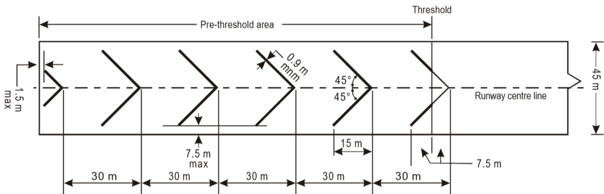
Figure 7-2. Pre-threshold marking
