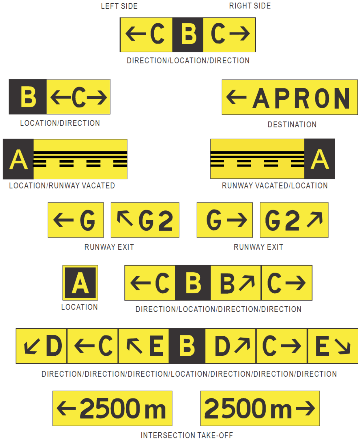
Figure 5-31. Information signs
