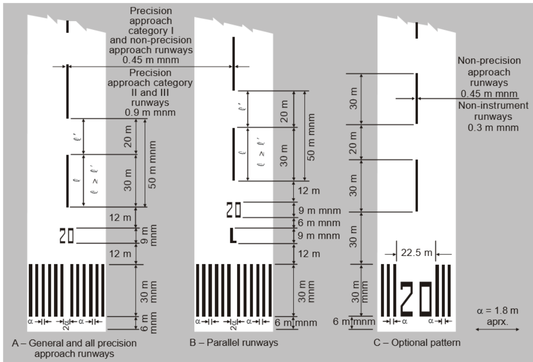
Figure 5-2. Runway designation, centre line and threshold markings
