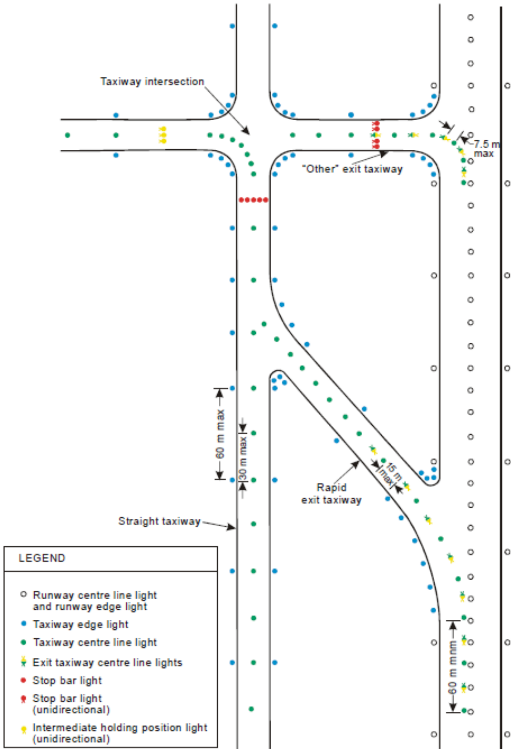
Figure 5-26. Taxiway lighting
