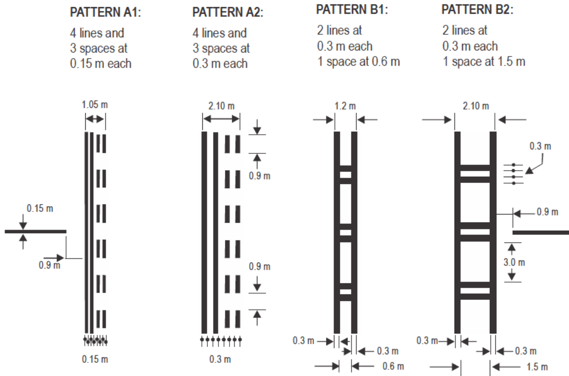
Figure 5-8. Runway-holding position markings Note.— Patterns A1 and B1 are no longer valid after 2026.
