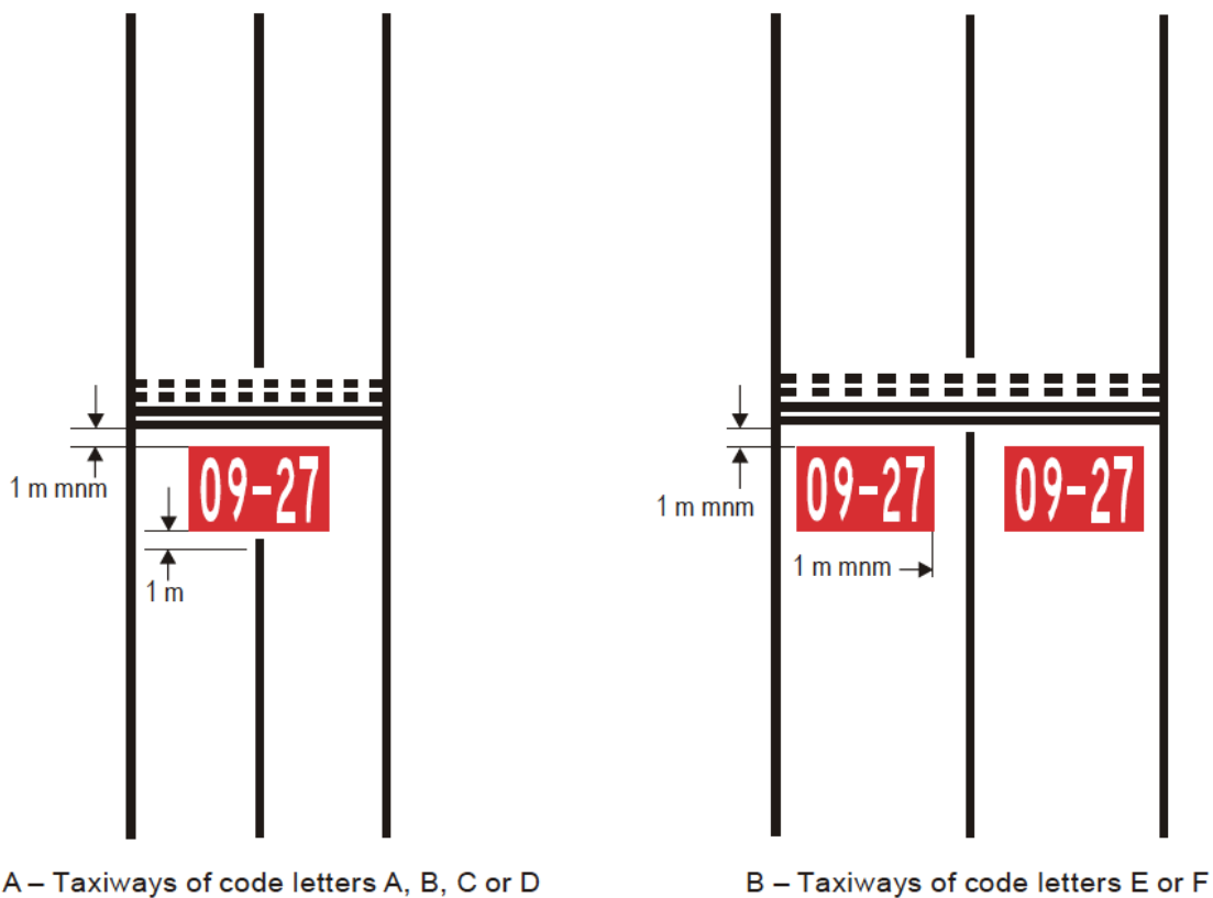
Figure 5-10. Mandatory instruction marking
