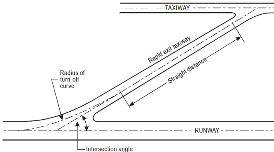
Figure 3-3. Rapid exit taxiway
