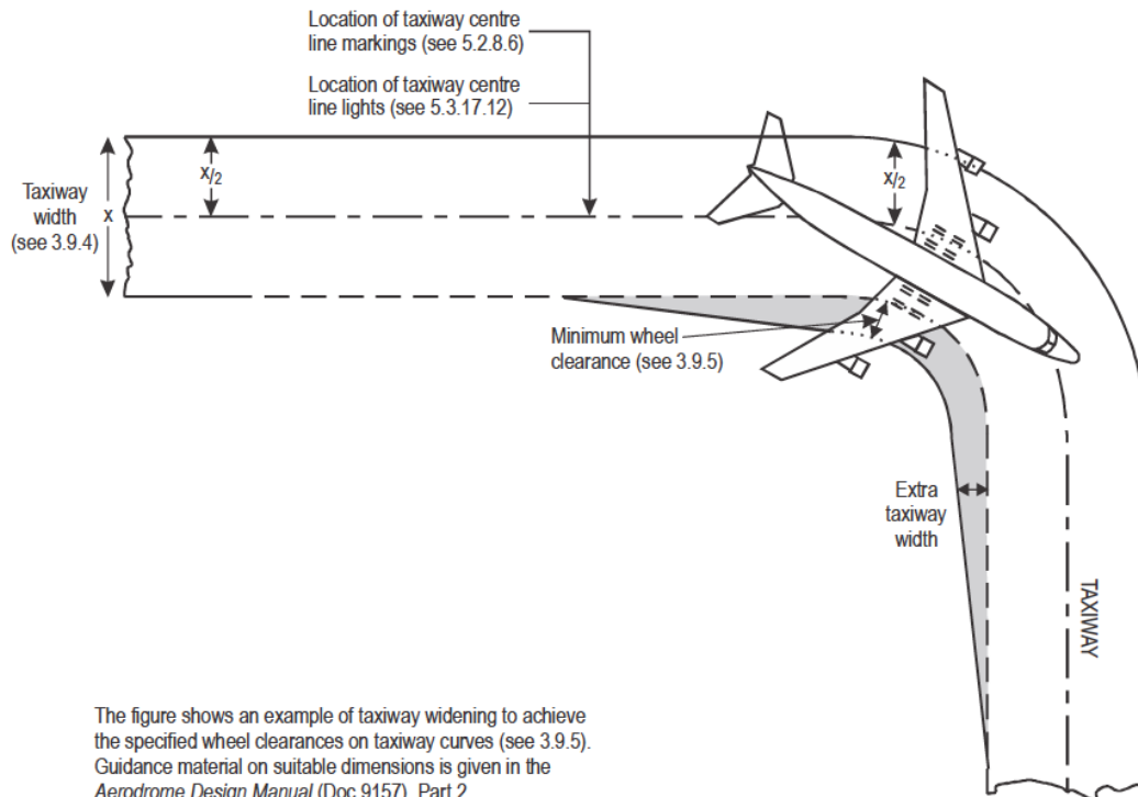
Figure 3-2. Taxiway curve
