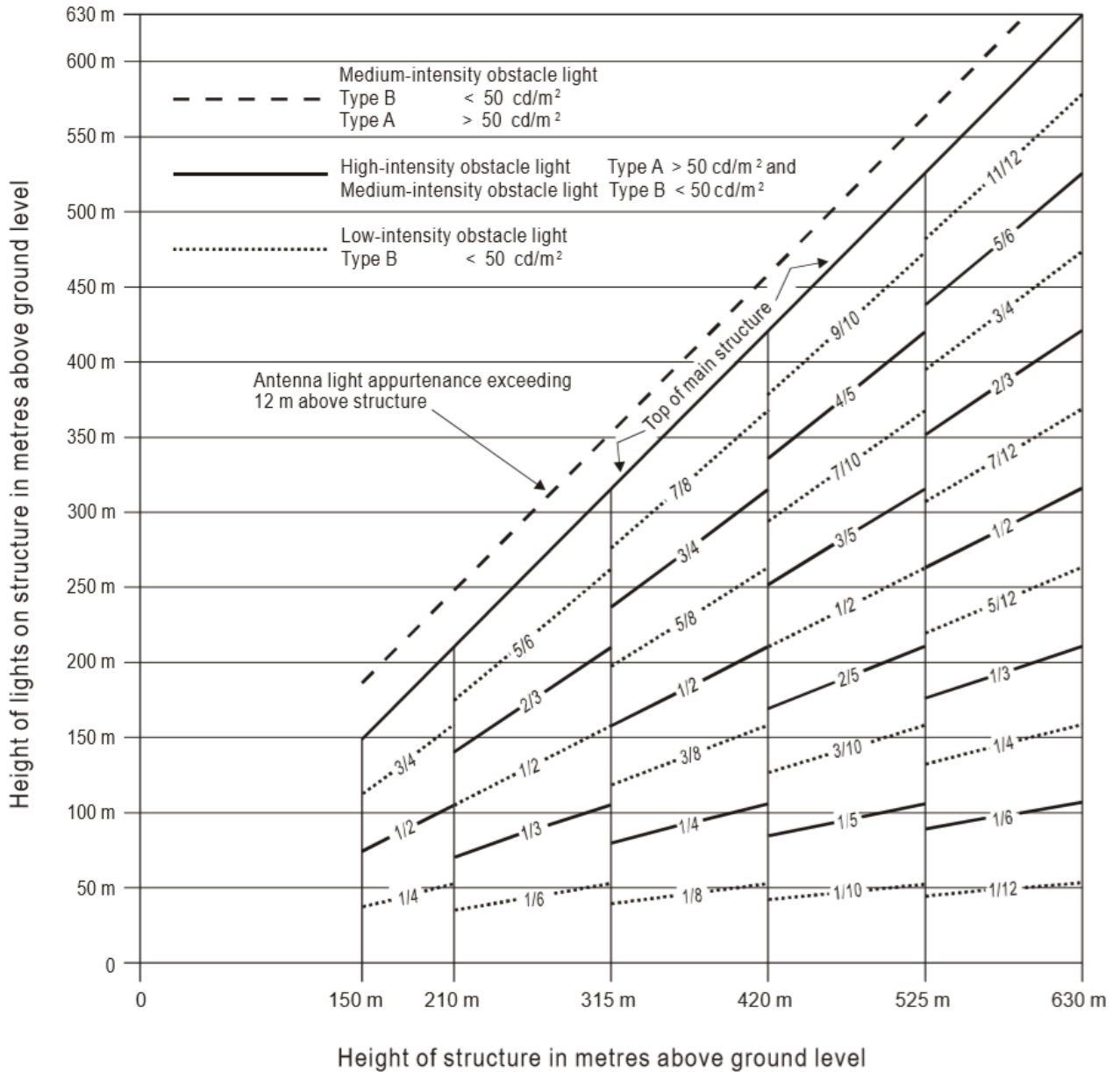
Figure A5-5. High-/medium-intensity dual obstacle lighting system, Type A/Type B
