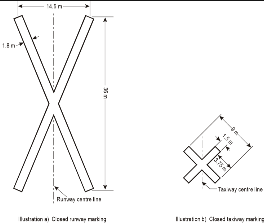
Figure 7-1. Closed runway and taxiway markings
