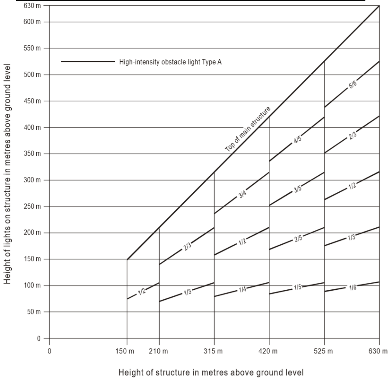
Figure A5-4. High-intensity flashing-white obstacle lighting system, Type A
