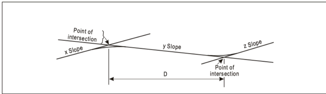
Figure A-2. Profile Centre line of runways
