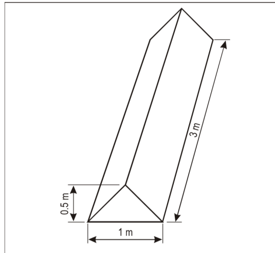
Figure 5-34. Boundary marker
