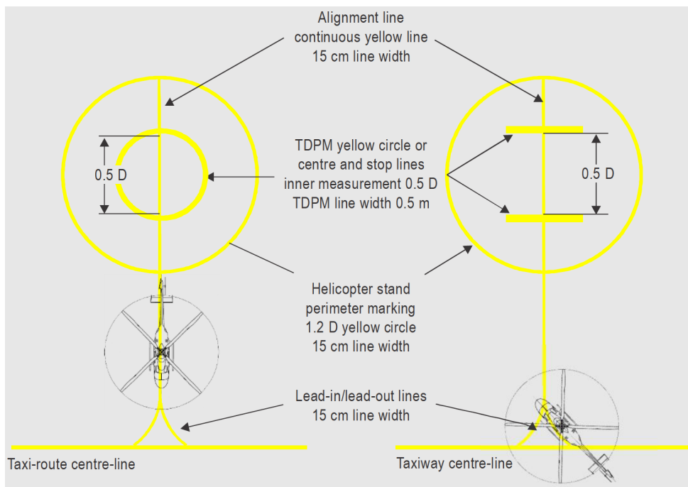
Figure 5-9. Helicopter stand markings
