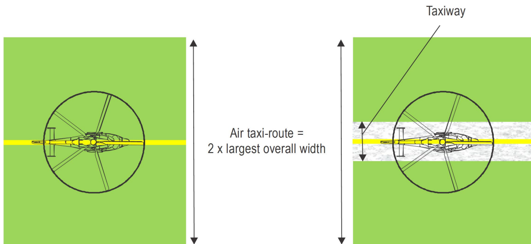
Figure 3-4. Helicopter air taxi -route and combined air taxi-route/taxiway
