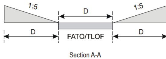
Figure 4-10. Amidship's location — shipboard heliport obstacle limitation surfaces
