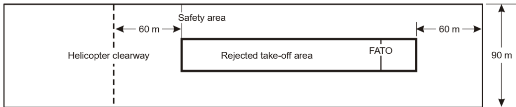
Figure A-1. Safety area for instrument FATO
