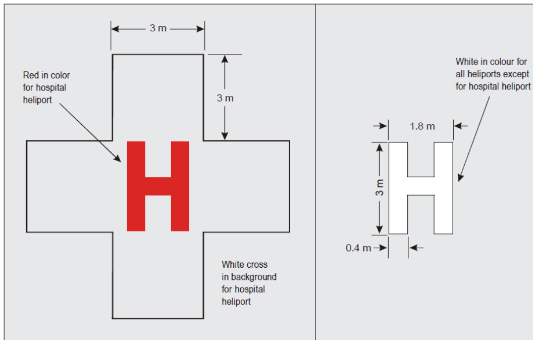
Figure 5-4. Hospital heliport identification and heliport identification marking
