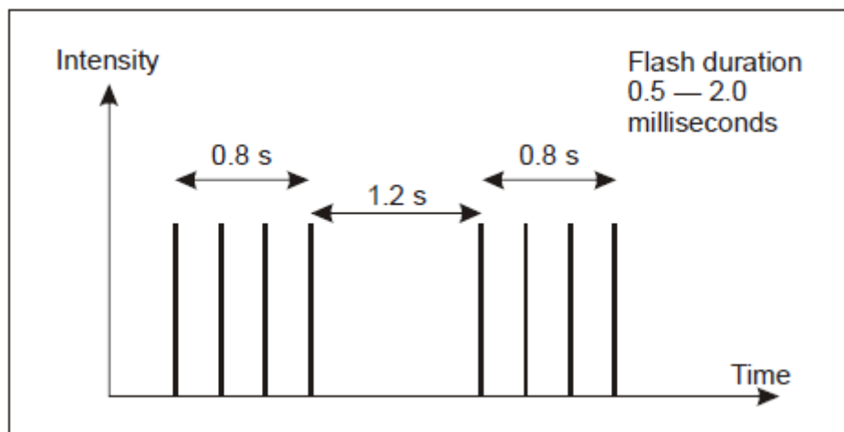
Figure 5-11. Heliport beacon flash characteristics
