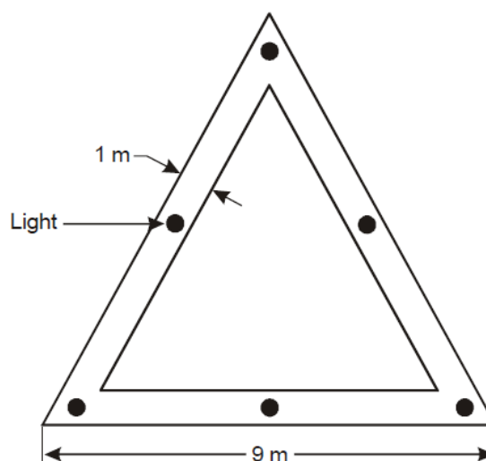
Figure 5-7. Aiming point marking
