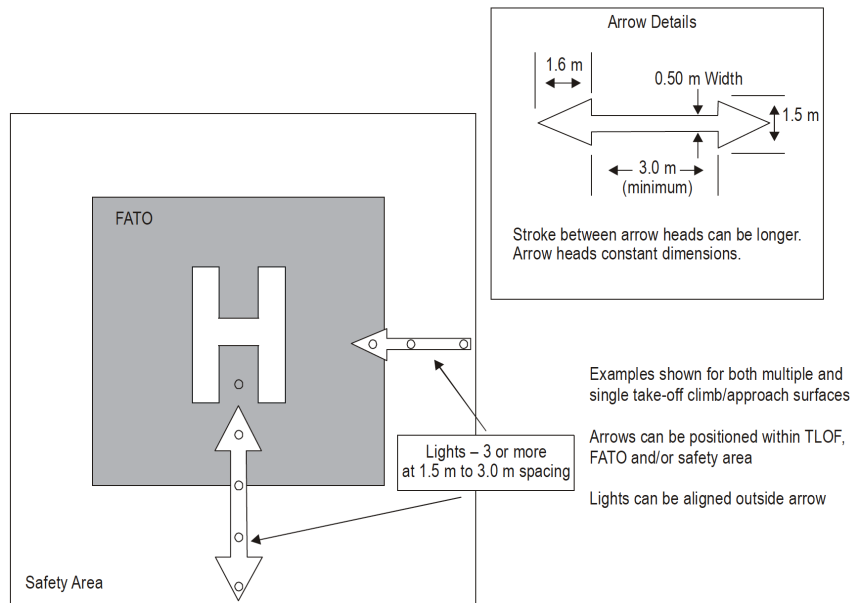
Figure 5-10. Flight path alignment guidance markings and lights
