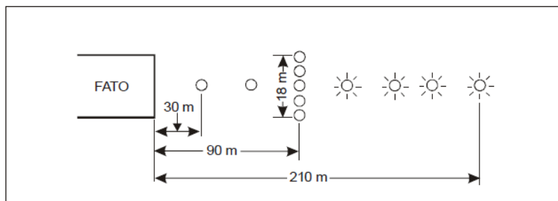
Figure 5-13 – Approach lighting system
