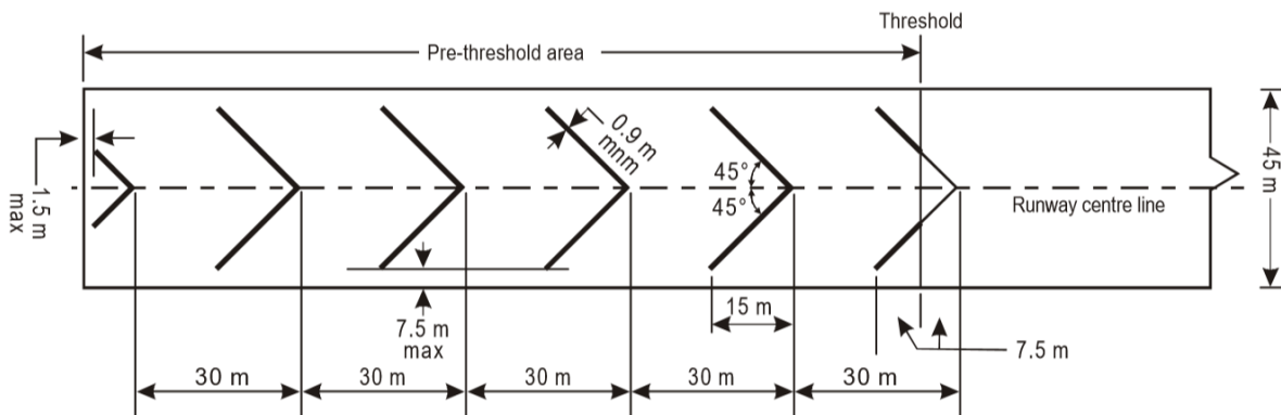
Figure 7-2. Pre-threshold marking
