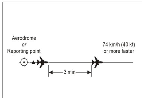
Figure 5-13. Three-minute separation between aircraft on same track and same level
