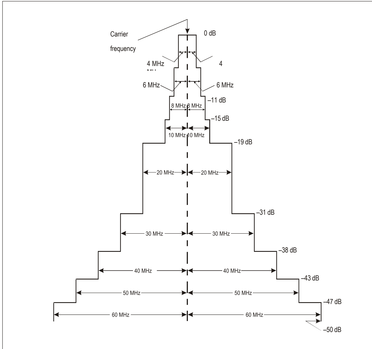
Figure 3-2. Required spectrum limits for interrogator transmitter
