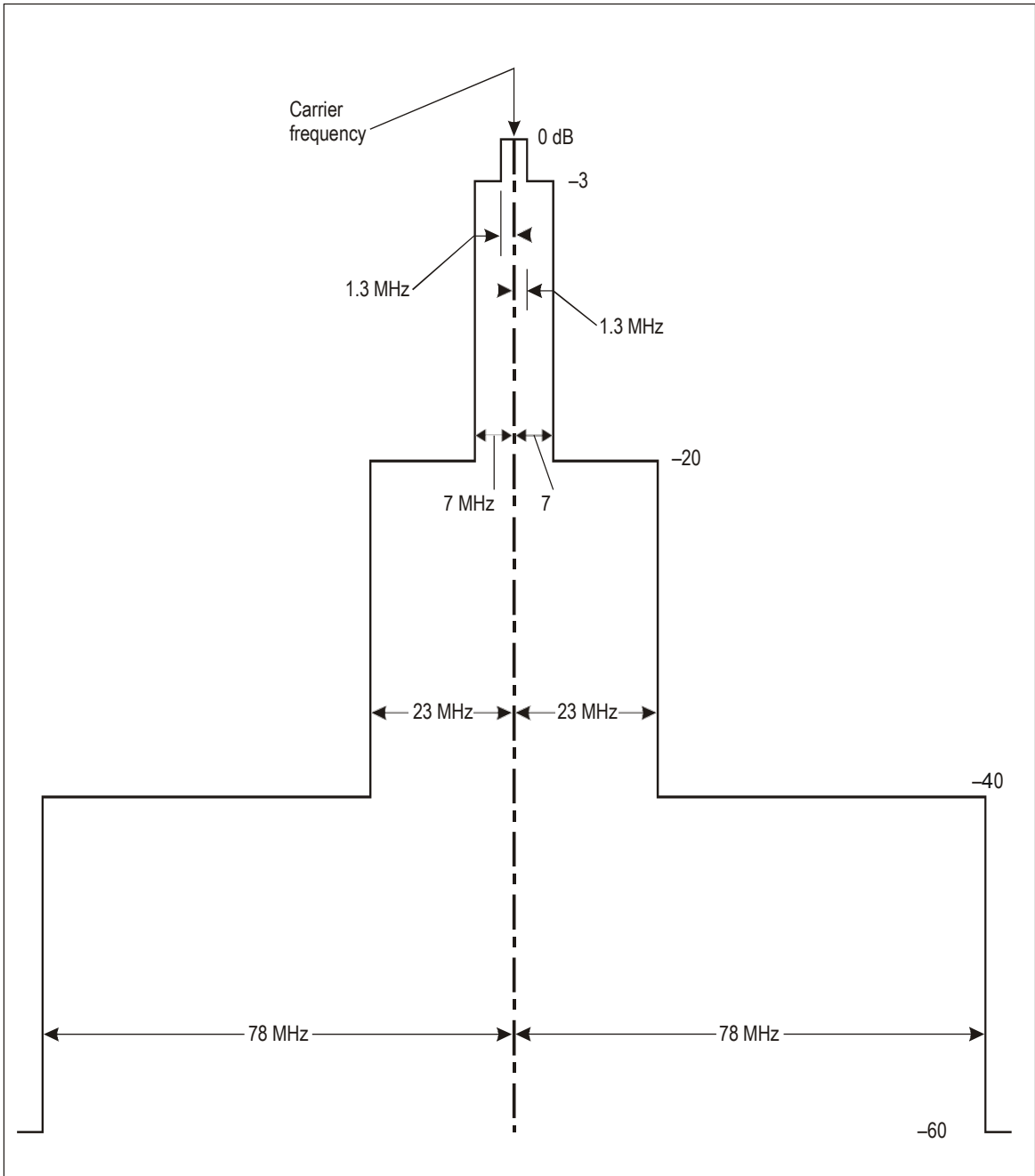
Figure 3-5. Required spectrum limits for transponder transmitter
