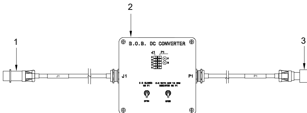
Figure 3 – Main Parts
