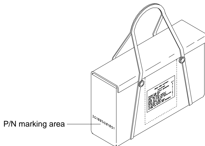
Figure 2 – P/N marking area
