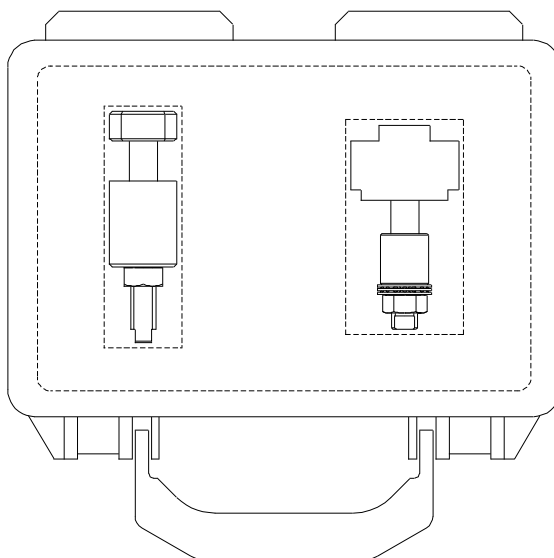
Figure 1 – Tool kit, gimbal / torque tube bushings repl. for MGB equipped with AGB system
