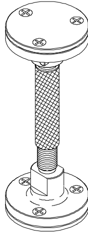
Figure 1 – Tool, retractor assy, M/R pitch control lever inst
