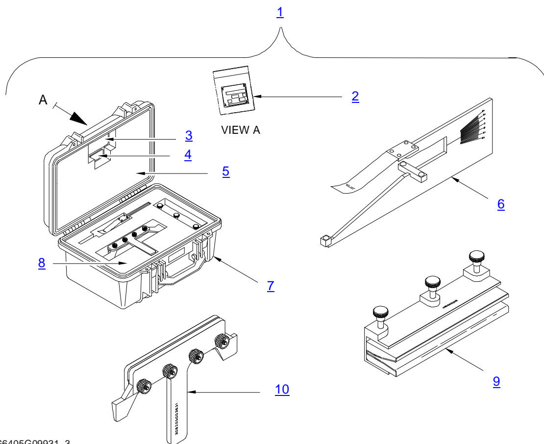
Figure 5 – Spare Parts
