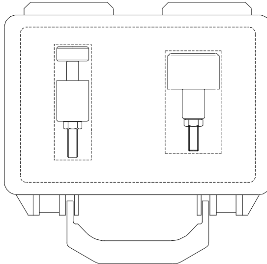
Figure 1 – Tool kit, gimbal / torque tube bushings repl.
