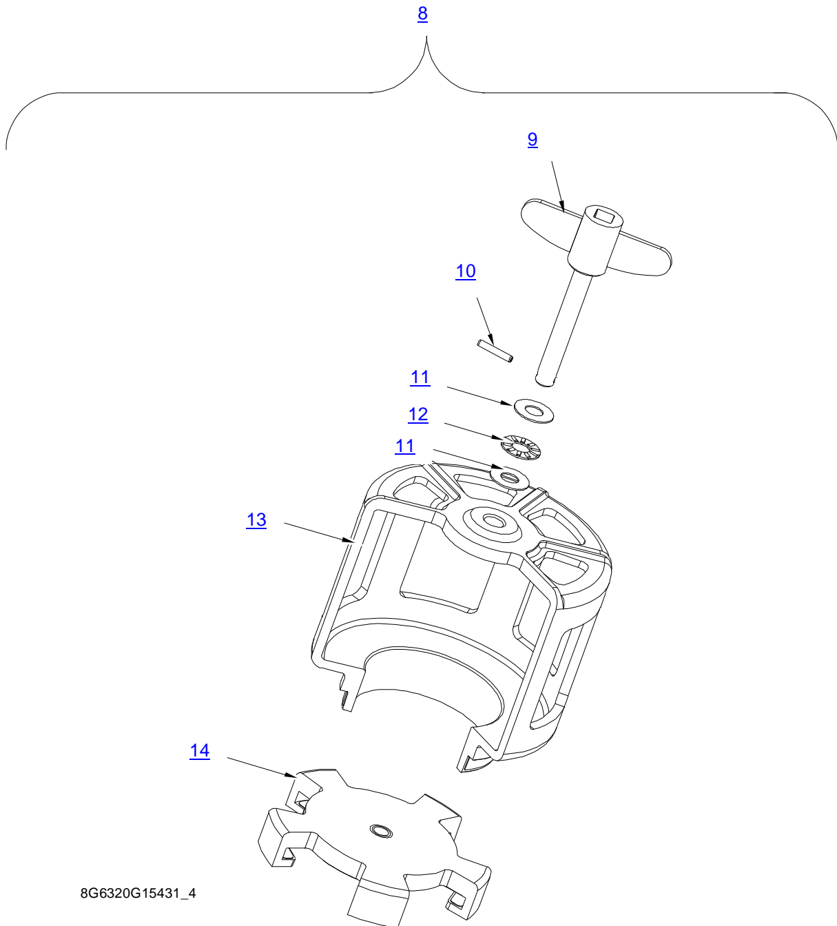
Figure 6 – Spare Parts
