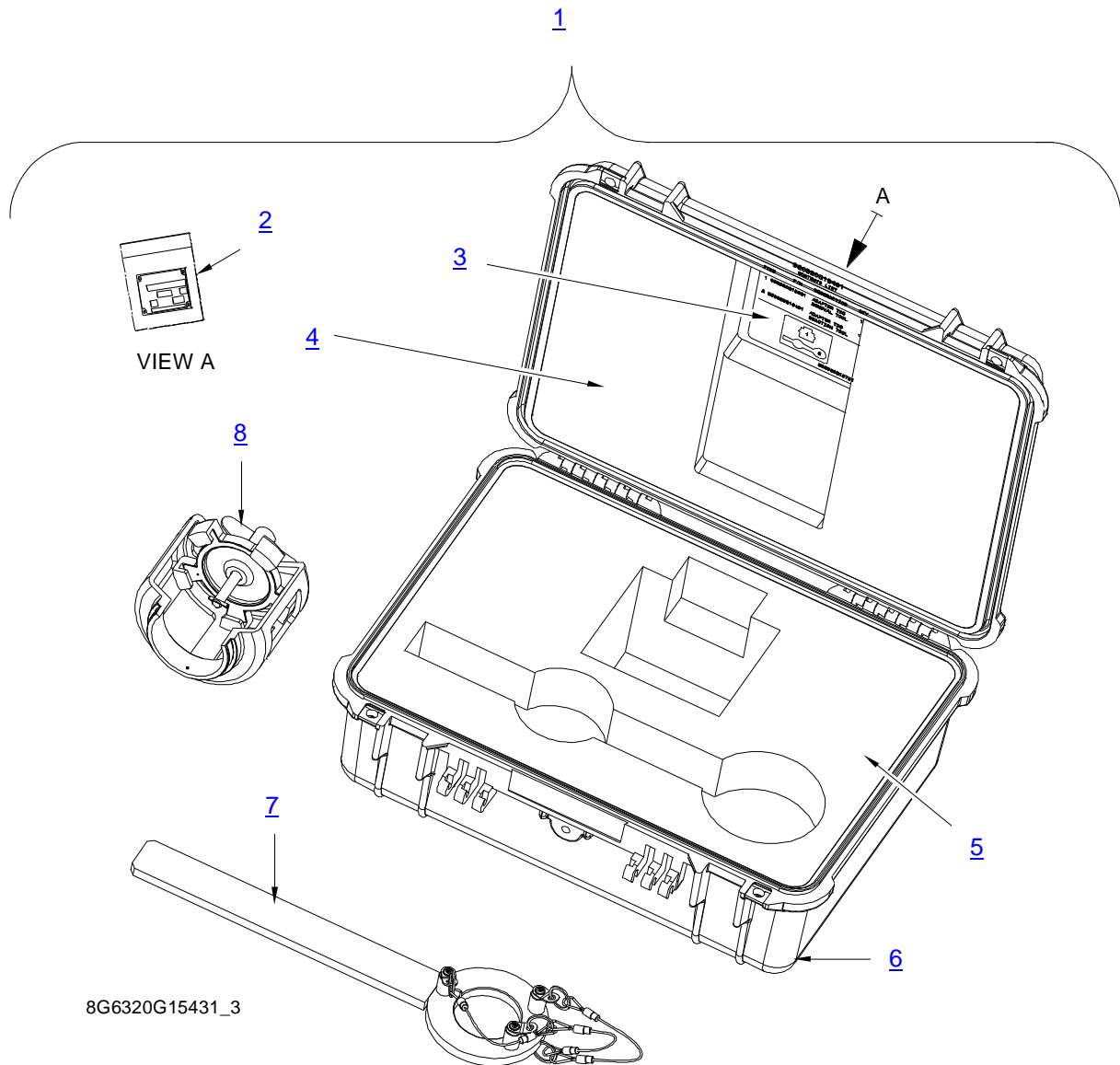
Figure 5 – Spare Parts
