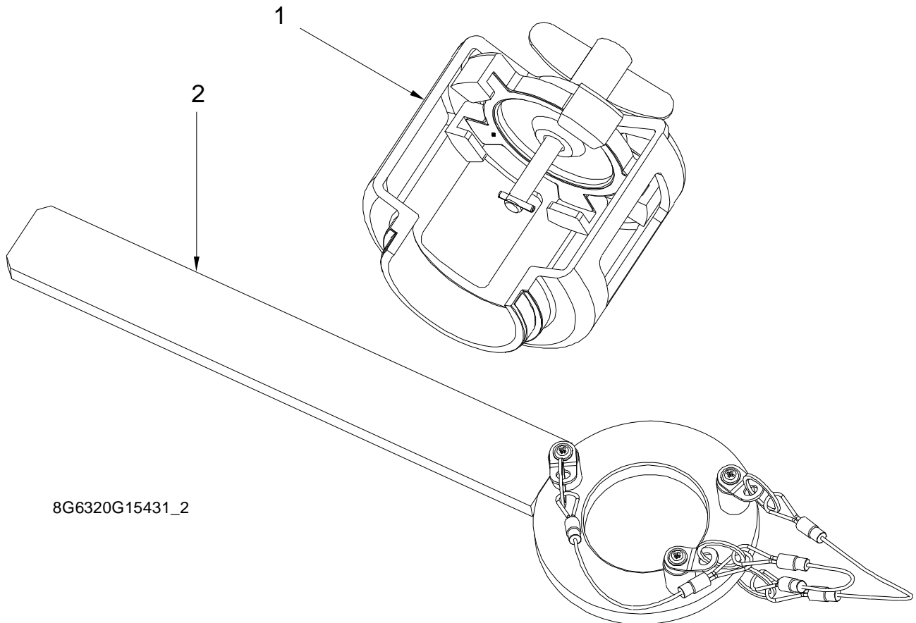
Figure 3 – Main Parts
