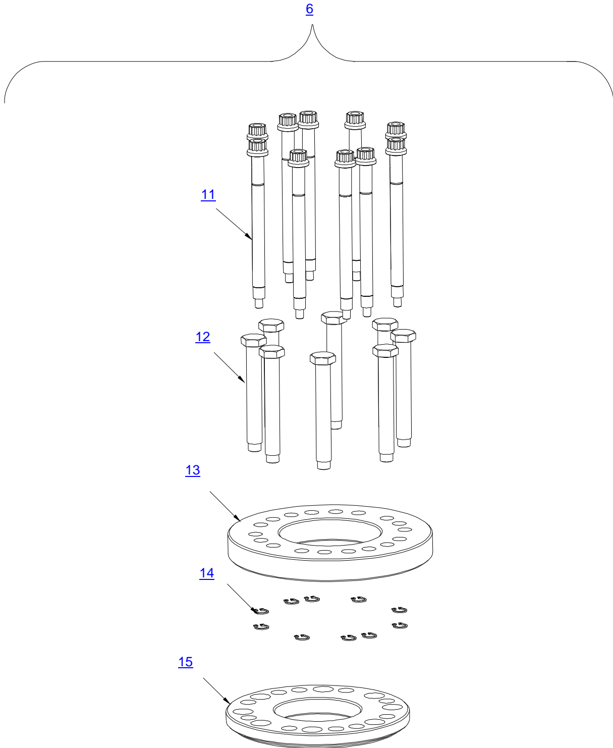
Figure 6 – Spare Parts
