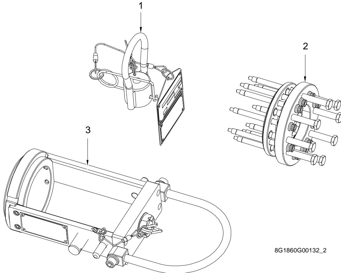
Figure 3 – Main Parts
