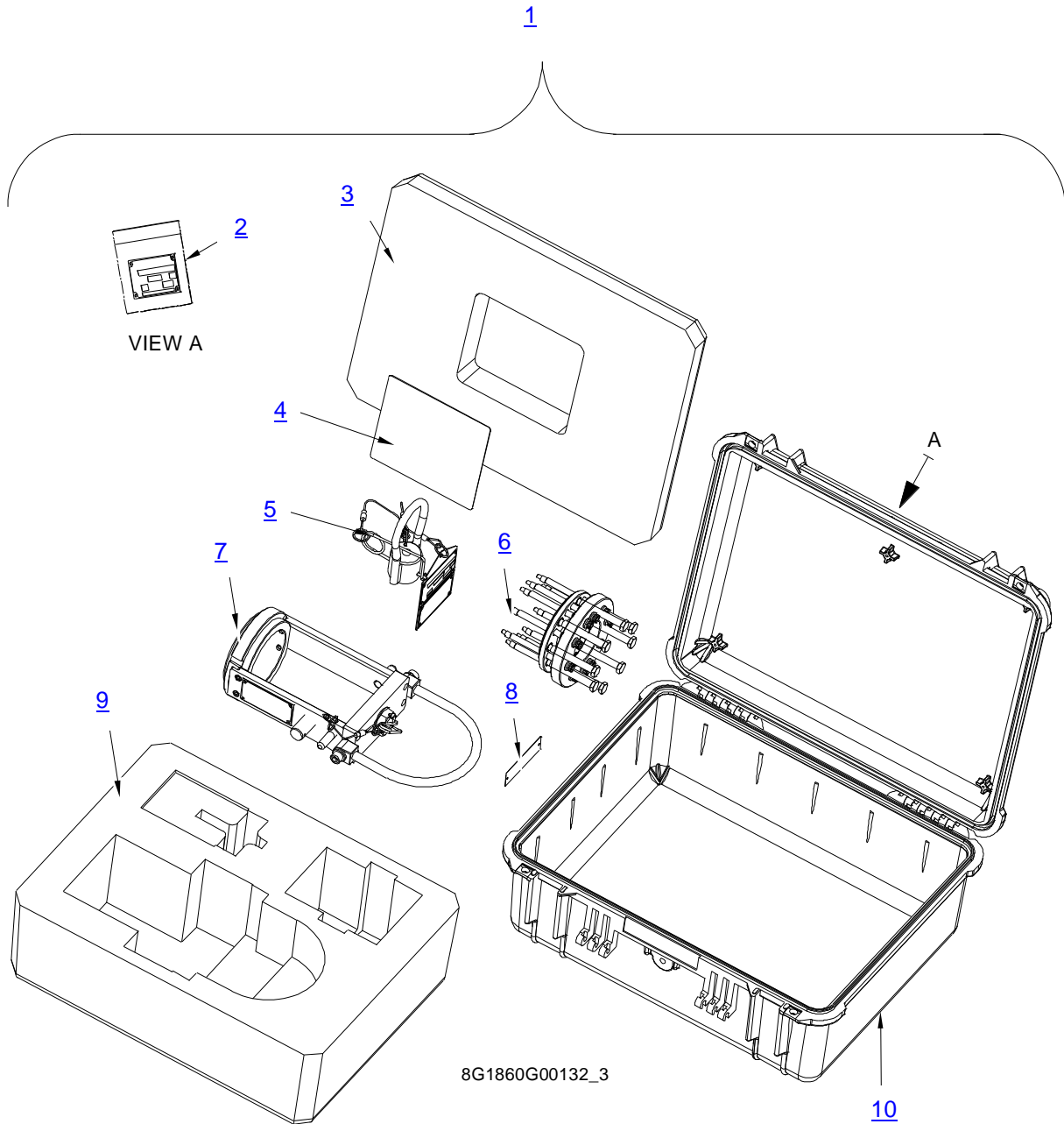
Figure 5 – Spare Parts
