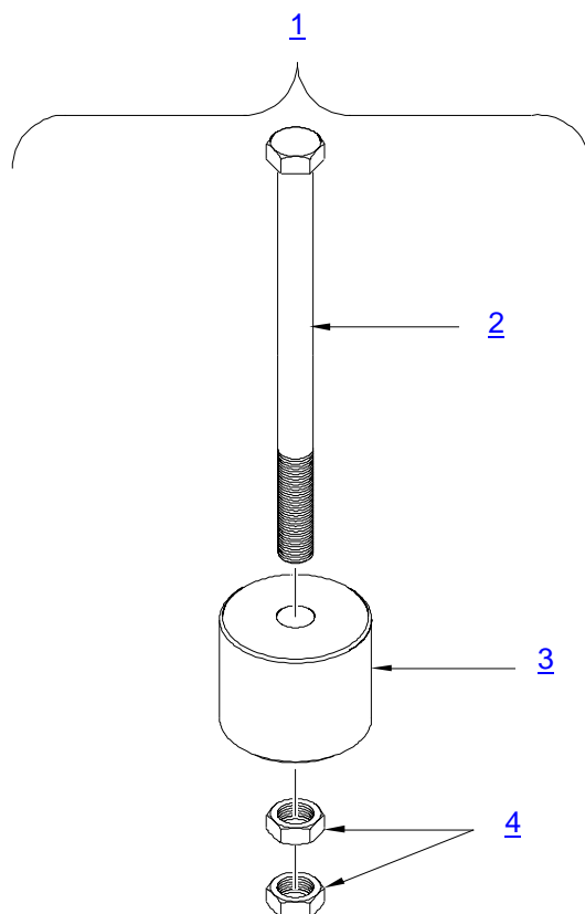
Figure 5 – Spare Parts
