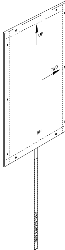
Figure 1 – Engine Air Intake Cover, RH
