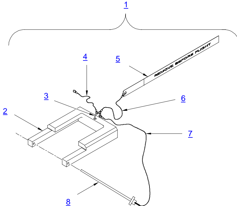
Figure 5 – Spare Parts
