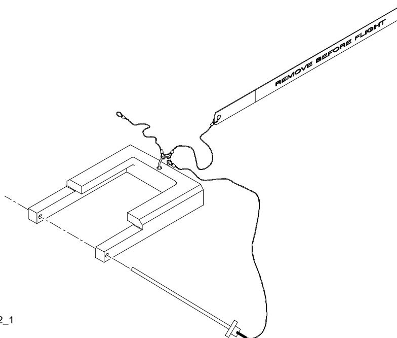
Figure 1 – T/R blades flapping block
