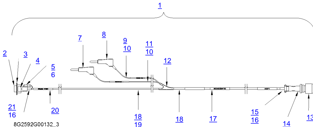
Figure 5 – Spare Parts
