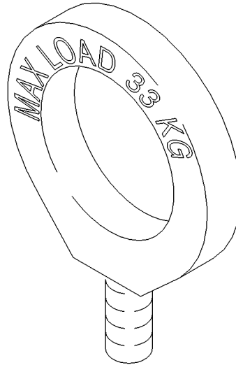
Figure 1 – Eyebolt, tail gearbox lifting
