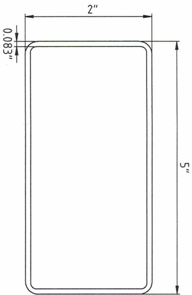
CROSS-SECTIONAL VIEW
