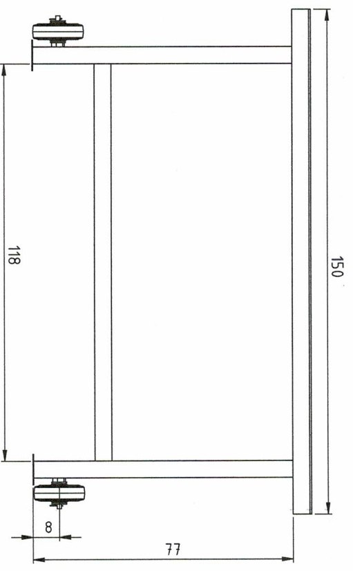
FRONT VIEW
