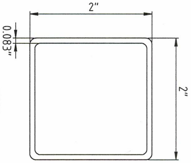
CROSS-SECTIONAL VIEW
