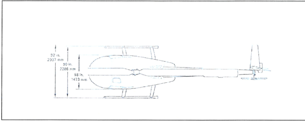
FIGURE 2: TOP AREA
