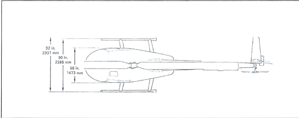
FIGURE 2: TOP AREA
