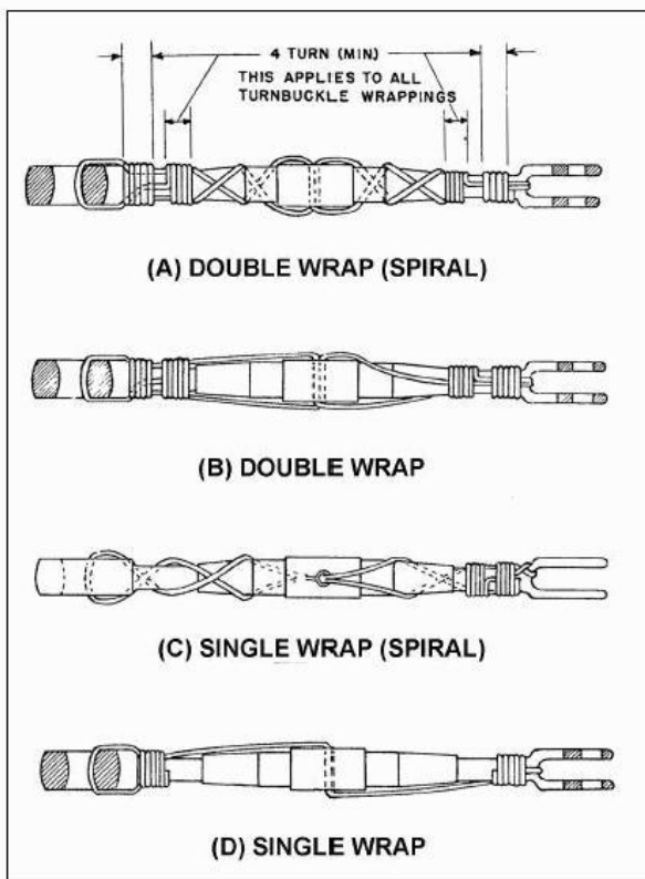
FIGURE 7-24. Safelying turnbuckles.
