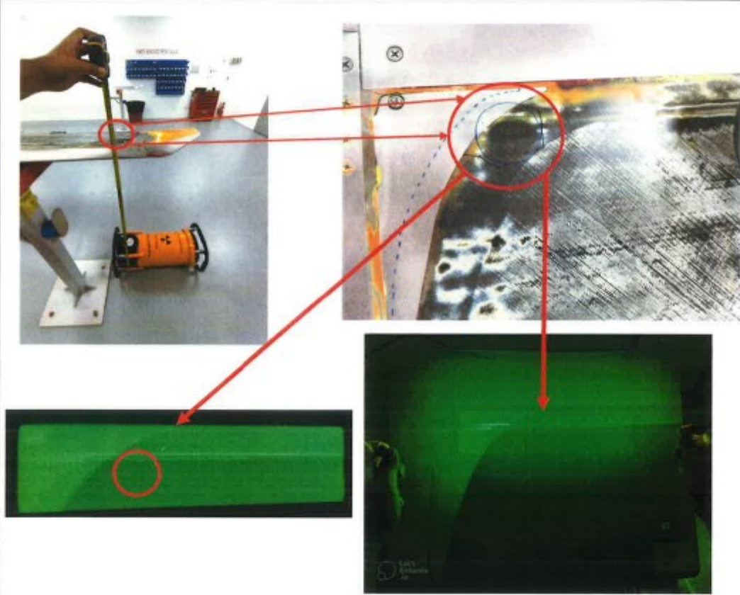
FIGURE 1: INTEREST AREA SHOWN WITHOUT ANY DEFECT INDICATION (EXPOSURE NO.0129)
