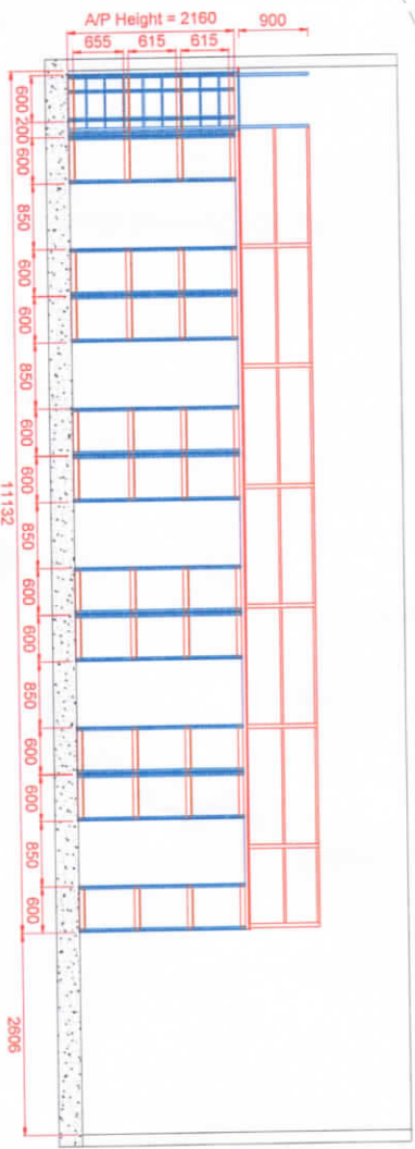
Front View 11132 SCALE: 1/100
