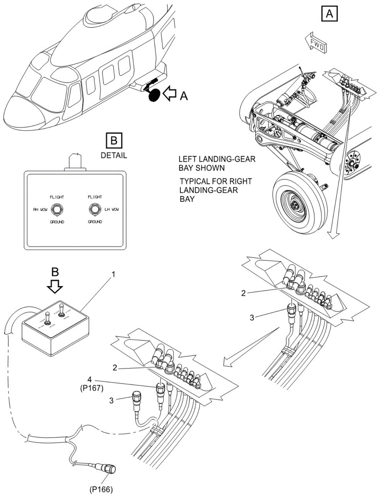
Figure 1 MLG microswitches test box (Liebherr landing gear) - Disconnect procedures
